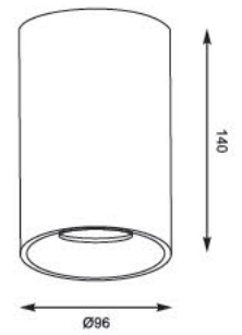
DEEP SL Spot 1. 89313 1°GU10 MAX 50W aluminium black/gold
