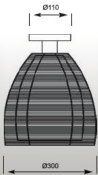
PICO: Ceiling 1. MX9023-1L (silver), 2. MX9023-1L (black), Pendant 1. MD9023-3B (silver), 2. MD9023-3B (black)
